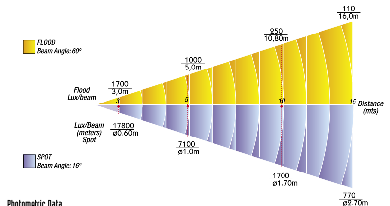
Photometric Data With lamp EGT 1000W-120V
